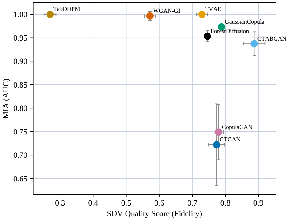
Adult: SDV Quality Score (Fidelity) vs MIA (AUC)
